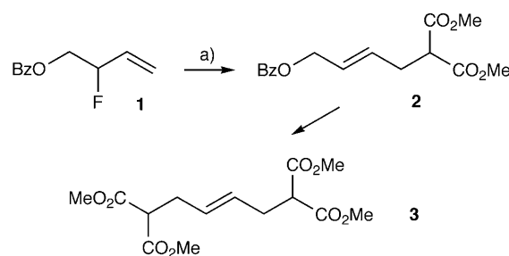
Scheme 2. Allylic alkylation of allylic fluoride 1 : a) CH 2 (CO 2 Me) 2 (3 equivalents), BSA (3 equivalents), [{Pd(η 3 -C 3 H 5 )Cl} 2 ] (10 mol %), PPh 3 (40 mol %), CH 2 Cl 2 , room temperature, 56%.
